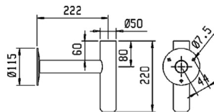
Wall support SK-5M
